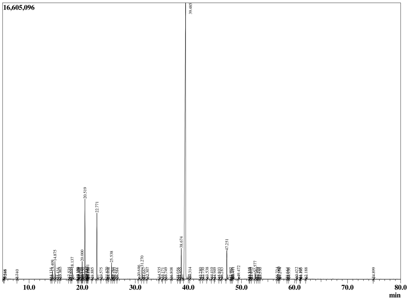
Chromatogram Origanum vulgare
